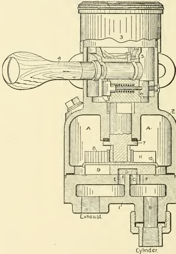
Fig. 93. Section of Air Operating Valve
